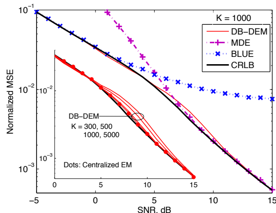
Fig. 1. NMSE vs. SNR for the DB-DEM, MDE, BLUE and centralized EM estimators. The CRLB is depicted as a reference.
