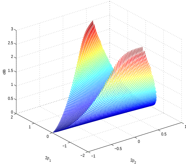
Fig. 1. Prediction gain of a first-order PLR predictor with an MA(2) input process.
