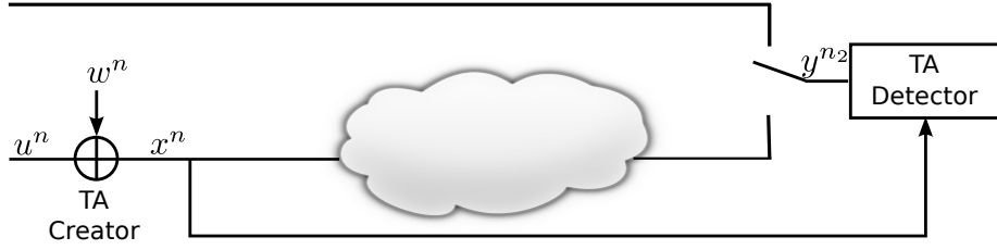
Figure 2.1: Flow correlation problem
