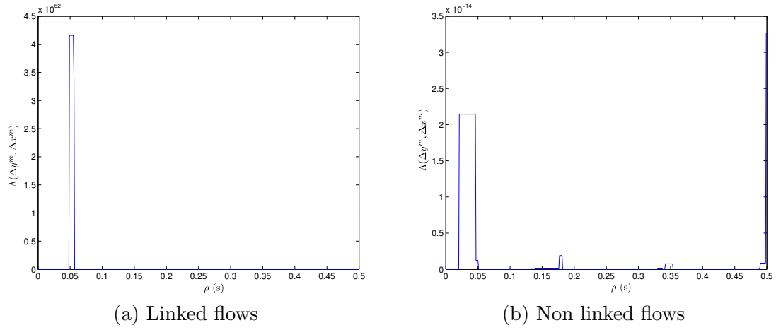
Figure 6.9: Synchronization in Scenario A with n = 6 .
