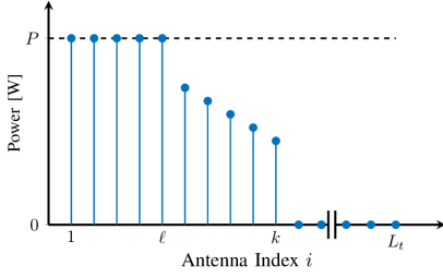
Fig. 3: General form of the power allocation coefficients |f_i|^2 .
