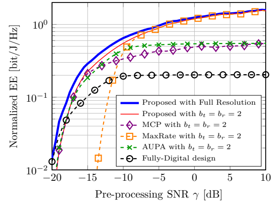
Fig. 7: Comparison of the EE performance vs. pre-processing SNR \gamma achieved with the proposed design with full and finite resolution PSs, and that exhibited by MCP, MaxRate, AUPA, and Fully-Digital benchmarks for \alpha = 0 .
