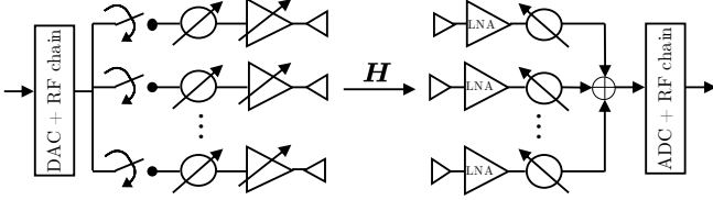
Fig. 2: Analog beamforming system model adopted in this work. The transmit beamformer is composed of switches, phase shifters, and VGAs; the receive beamformer comprises fixed-gain low-noise amplifiers and phase shifters.
