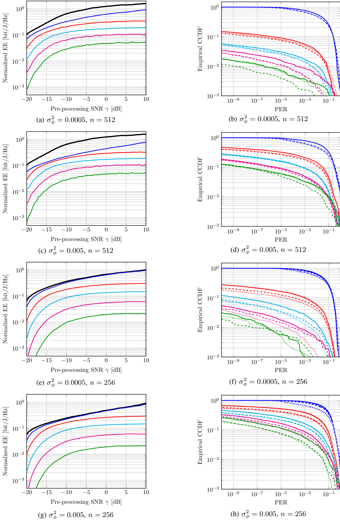
Fig. 11: Robustness evaluation of the proposed design with L_t = 32 and b_t = b_r = 2 bits, for packet size n = \{256, 512\} , \sigma_\beta^2 = 10^{-1} , \sigma_\theta^2 = 0.005 , and \sigma_\phi^2 \in \{0.005, 0.0005\} . In all cases, the performance of the full-resolution design under perfect CSI is depicted in black, and different values of the relative uncertainty have been tested: \alpha = 0 (blue), \alpha = 0.25 (red), \alpha = 0.5 (cyan), \alpha = 0.75 (magenta), and \alpha = 1 (green). The empirical CCDFs are shown at different pre-processing SNRs: \gamma = -5 dB (solid), \gamma = 0 dB (dashed), and \gamma = 5 dB (dotted). Results averaged over 10^4 Monte Carlo runs.
