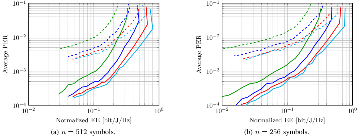
Fig. 12: EE-PER tradeoff curves for L_t = 32 and b_t = b_r = 2 bits, for \sigma_\beta^2 = 10^{-1} ; \sigma_\theta^2 = 0.005 ; different DoD error variance: \sigma_\phi^2 = 0.0005 (solid) and \sigma_\phi^2 = 0.005 (dashed); and different pre-processing SNR: \gamma = -10 dB (green) \gamma = -5 dB (blue), \gamma = 0 dB (red), and \gamma = 5 dB (cyan).
