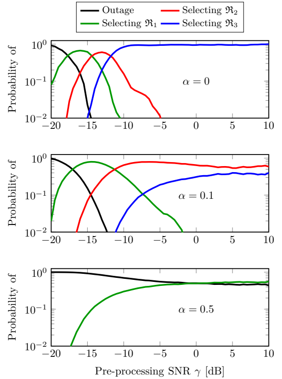
Fig. 10: Probability of using each encoder \mathfrak{R}_{1 \leq q \leq 3} and probability of outage vs. pre-processing SNR \gamma with full-resolution PSs for different values of \alpha .
