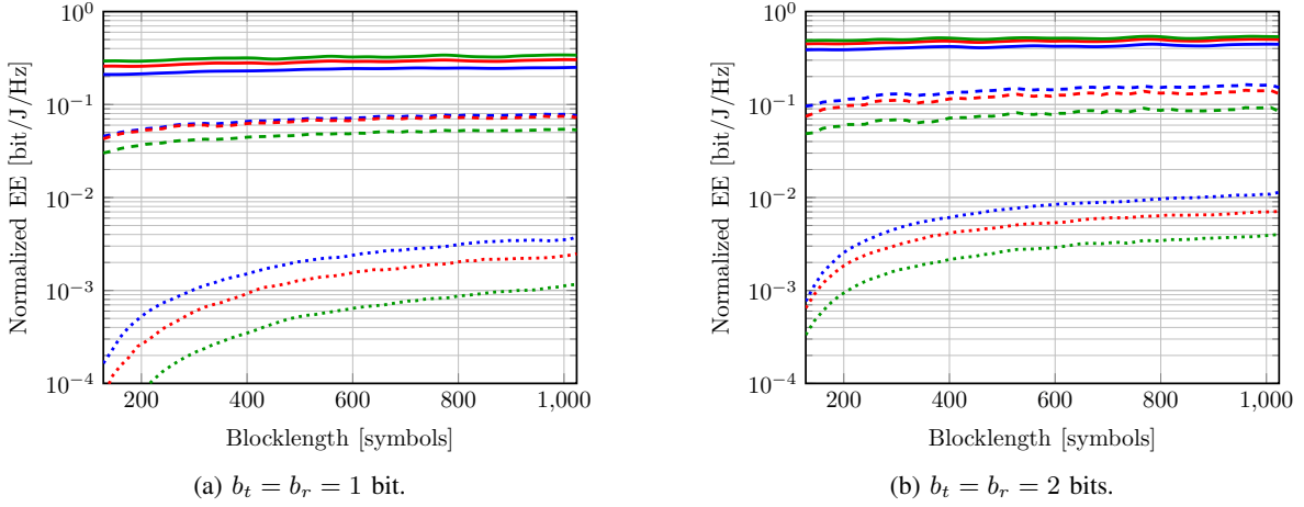
Fig. 6: EE versus the blocklength with quantized PSs at pre-processing SNR \gamma = -5 dB. Results plotted for different relative uncertainties: \alpha = 0 (solid), \alpha = 0.1 (dashed), and \alpha = 0.5 (dotted); and for different number of transmit antennas: L_t = 32 (blue), L_t = 64 (red), and L_t = 128 (green).
