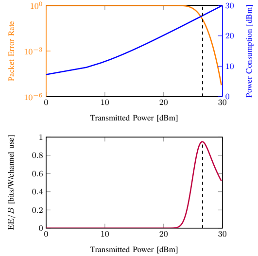
Fig. 1: Maximum-EE analog beamforming performance. Top: PER (as per [30]) and power consumption (as per [41]) vs. transmit power. Bottom: EE normalized by system bandwidth vs. transmit power. Setup: transmitter equipped with a 16-element fully analog array with unquantized phase shifters, per-antenna variable gain control, and a single channel encoder with rate R = 1/2 [see (1)]; single-antenna receiver. Packet length: 100 symbols. All channel paths have the same gain, such that the only design parameter is the power allocation, and the SNR depends only on transmit power.
