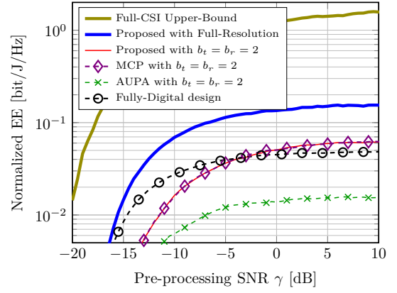
Fig. 9: Comparison of the EE performance vs pre-processing SNR \gamma achieved with the proposed design with full and finite resolution PSs and that exhibited by MCP and AUPA benchmarks for the case \alpha = 0.5 .
