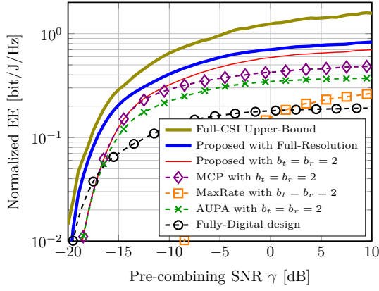
Fig. 8: Comparison of the EE performance vs. pre-processing SNR \gamma achieved with the proposed design with full and finite resolution PSs, and that exhibited by MCP, MaxRate, AUPA, and Fully-Digital benchmarks for \alpha = 0.1 .
