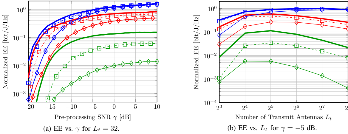
Fig. 5: Performance evaluation of the worst-case design proposed in Sec. III: (a) EE vs pre-processing SNR \gamma ; (b) EE vs number of transmit antennas L_t . In both cases, the EE is plotted for different relative uncertainties: \alpha = 0 (blue), \alpha = 0.1 (red), and \alpha = 0.5 (green). Different PSs resolutions are assessed: infinite (thick solid), b_t = b_r = 2 bits (dashed with square markers), and b_t = b_r = 1 bit (thin solid with diamond markers).
