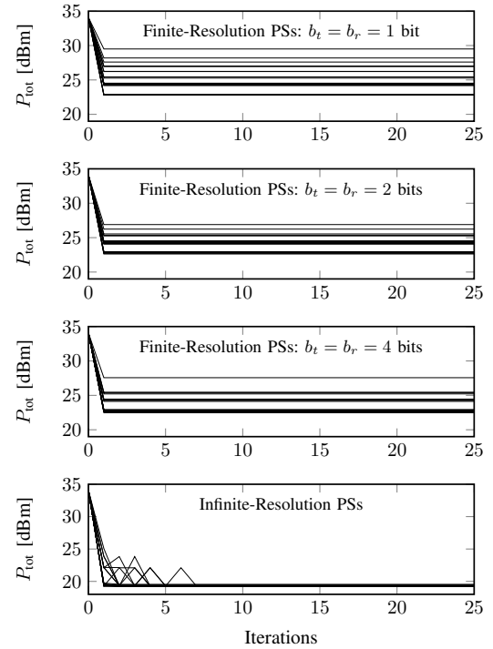
Fig. 4: Convergence of the proposed algorithm for different PS resolutions, with L_t = 128 , L_r = 16 , \gamma = 5 dB, and \delta^2 = 0.5 \|\hat{\mathbf{H}}\|_F^2 .
